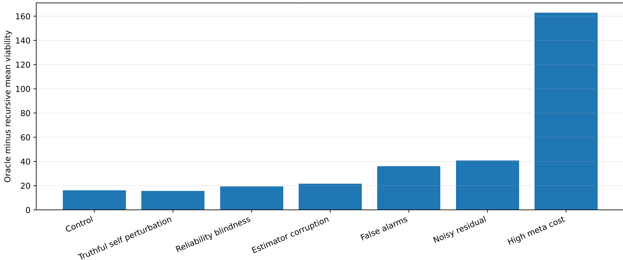
Remaining gap to oracle repair policy
